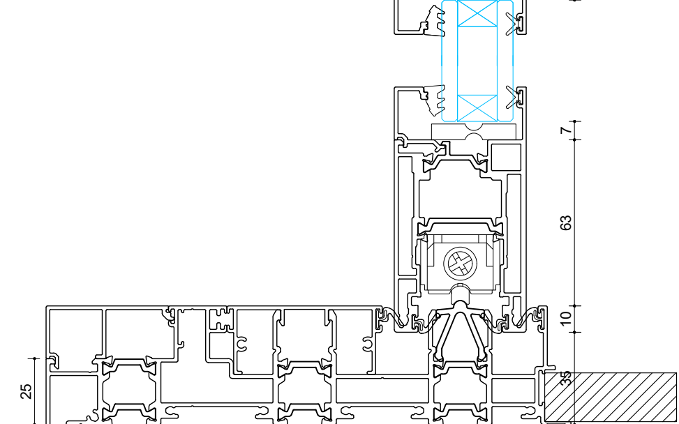
Section A Vertical Section Scale: 1:2
