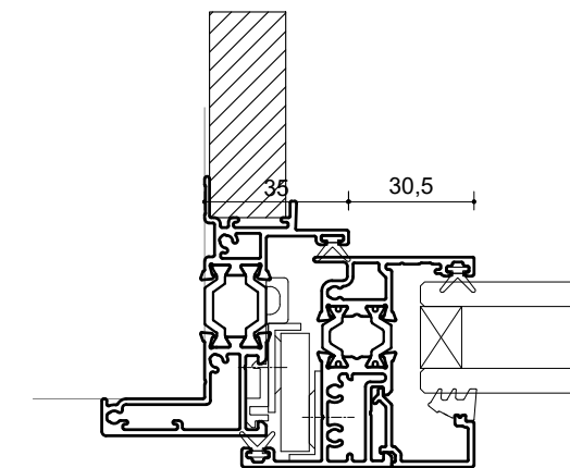
Section C Horizontal Section Scale: 1:2
